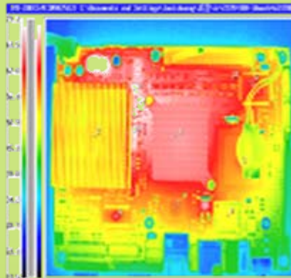
Thermal Testing
